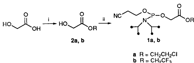
Scheme 1 Reagents: i, HOR, SOCl 2 ; ii, 2-cyanoethyl N,N,N',N' -tetraisopropylphosphorodiamidite, tetrazole, acetonitrile
