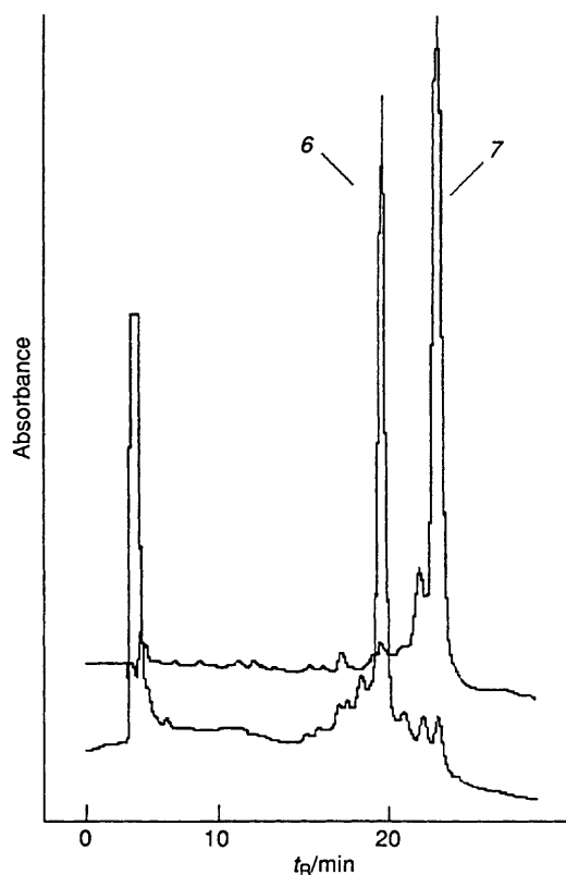
Fig. 1 Ion-exchange HPLC profiles of crude oligonucleotides 6 and 7 prepared with the aid of phosphoramidite 1a (gradient: System 1). The large peak at t R ~ 5 min refers to non-nucleosidic material.
