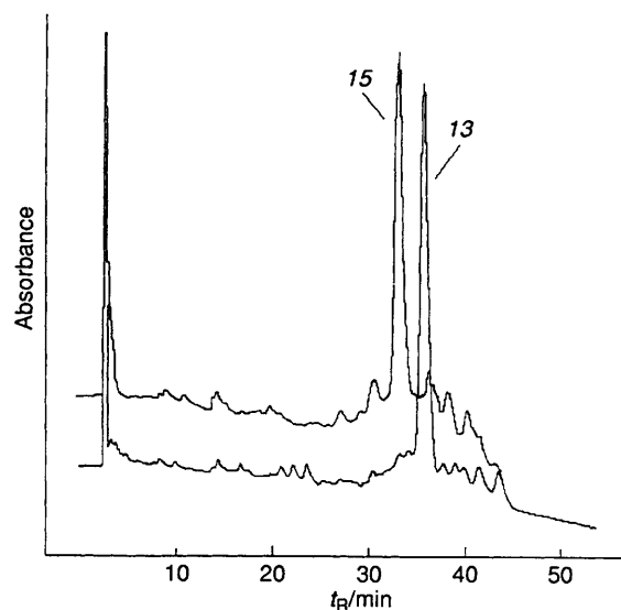
Fig. 2 Ion-exchange HPLC profiles of crude oligonucleotides 13 and 15 prepared with the aid of phosphoramidite 1b (gradient: System 2). The large peaks at t R ~ 5 min refer to non-nucleosidic material.
